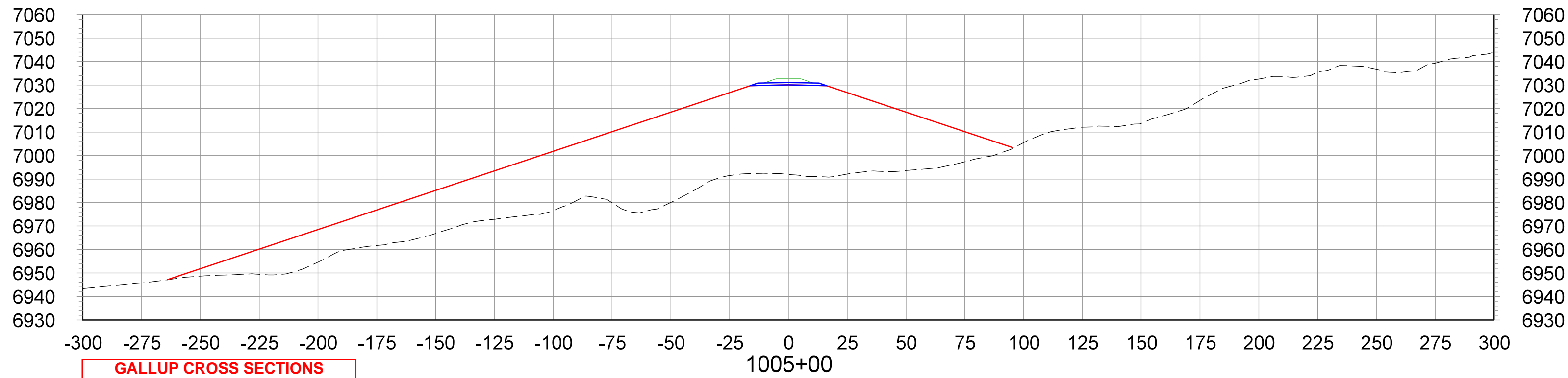
CROSS SECTIONS STA.1005+00 TO STA.1010+00
