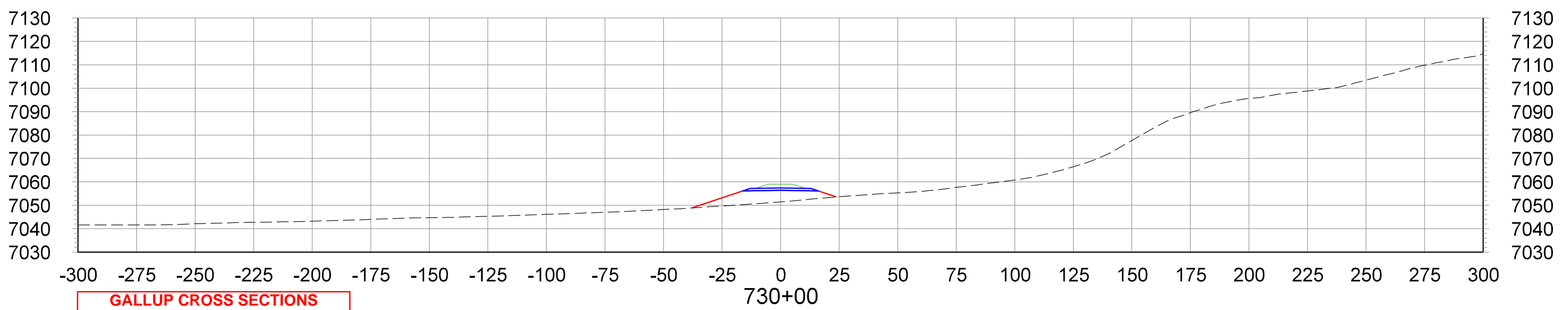
CROSS SECTIONS STA.730+00 TO STA.740+00
