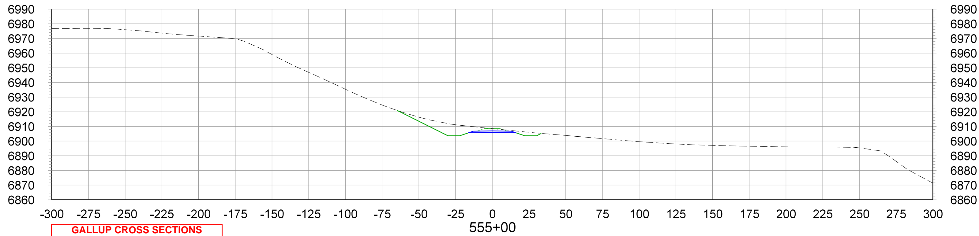
CROSS SECTIONS STA.555+00 TO STA.560+00
